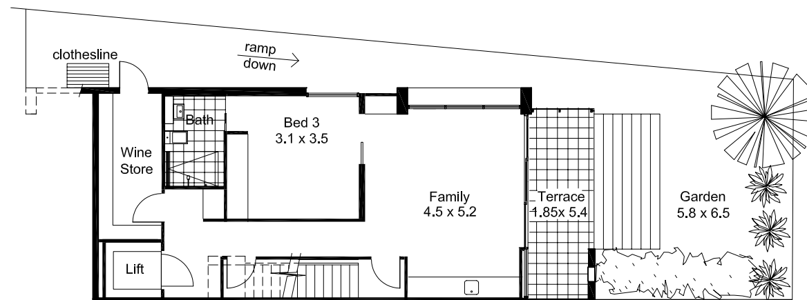
Townhouse 1 (Level 1)
